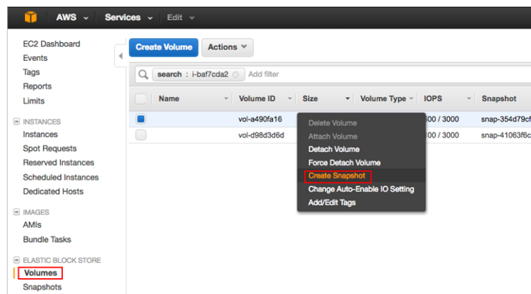
Figure 8: Create Snapshot
